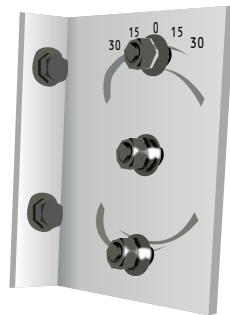
Millimeter adjustment assembly
